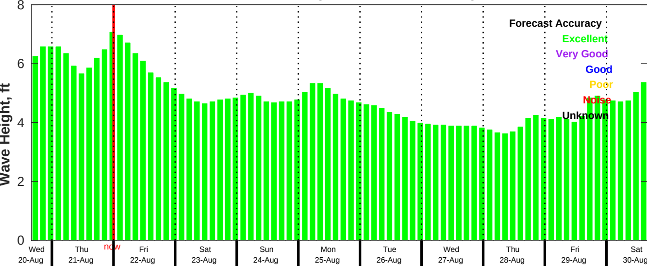
CMEMS Wave Forecast for NDBC 46011 from 20-Aug-2025 16:00:00 to 30-Aug-2025 16:00:00
