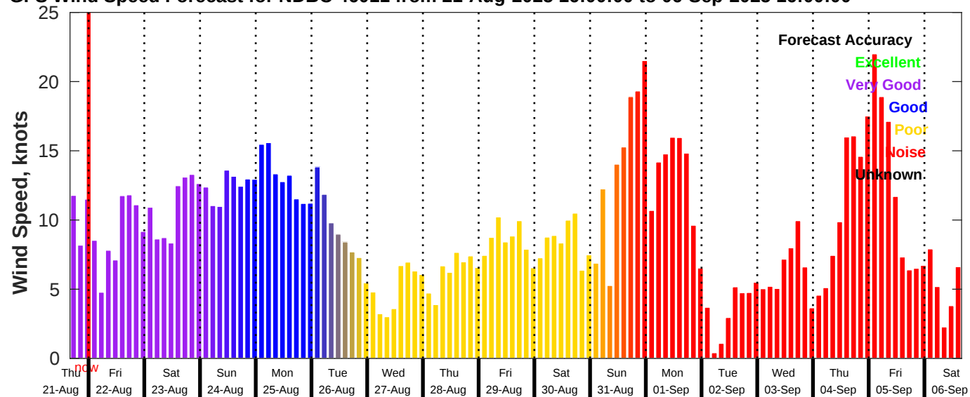
GFS Wind Speed Forecast for NDBC 46011 from 21-Aug-2025 16:00:00 to 06-Sep-2025 16:00:00
