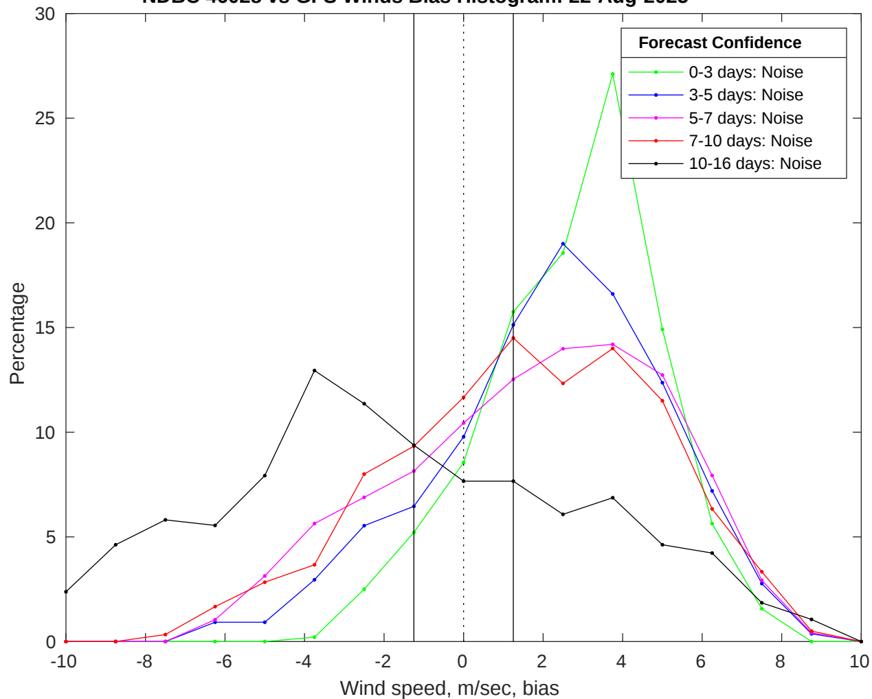
NDBC 46028 vs GFS Winds Bias Histogram: 22-Aug-2025
