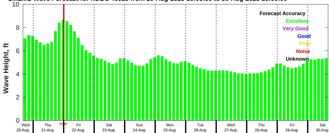
CMEMS Wave Forecast for NDBC 46028 from 20-Aug-2025 16:00:00 to 30-Aug-2025 16:00:00
