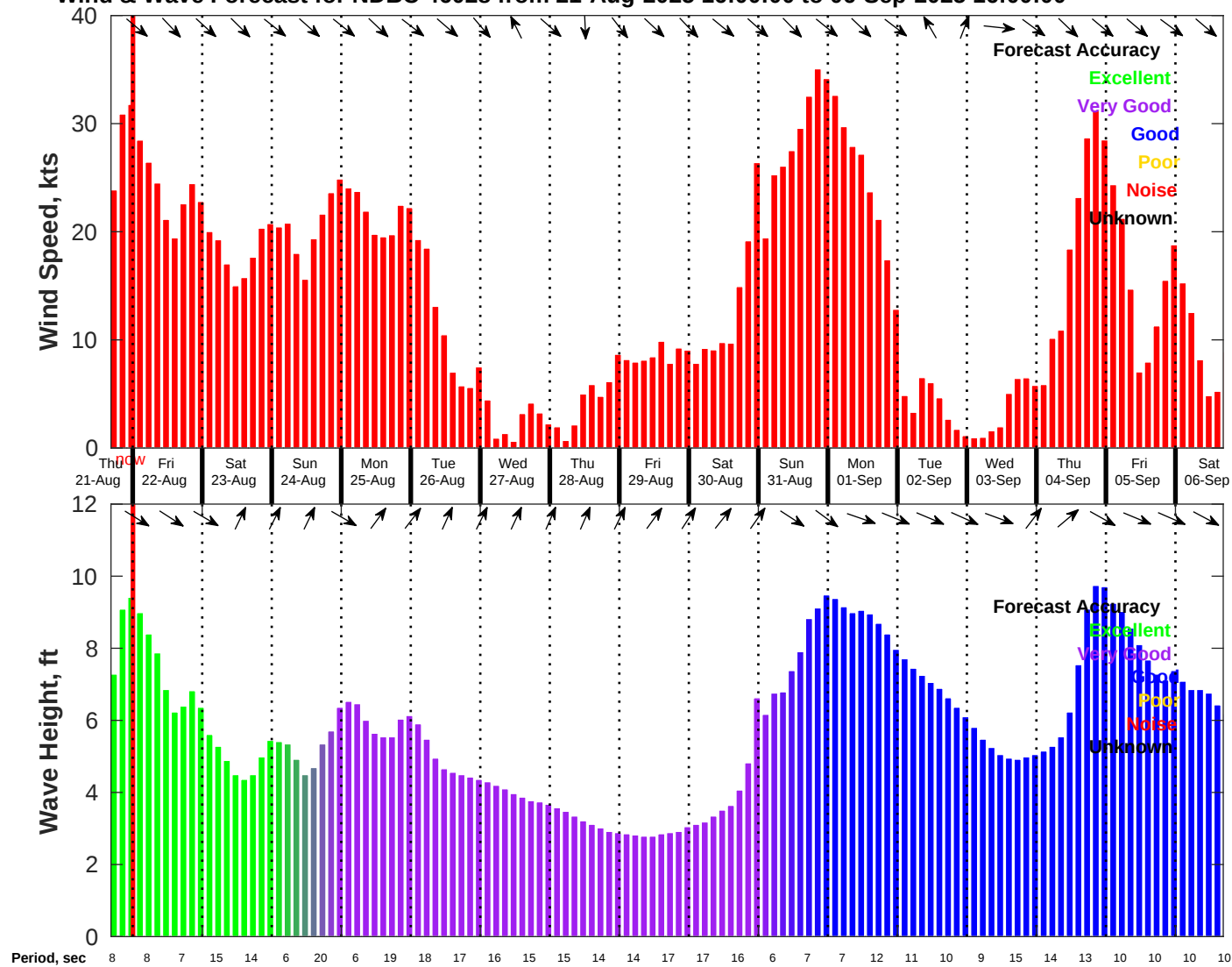
Wind & Wave Forecast for NDBC 46028 from 21-Aug-2025 16:00:00 to 06-Sep-2025 16:00:00
