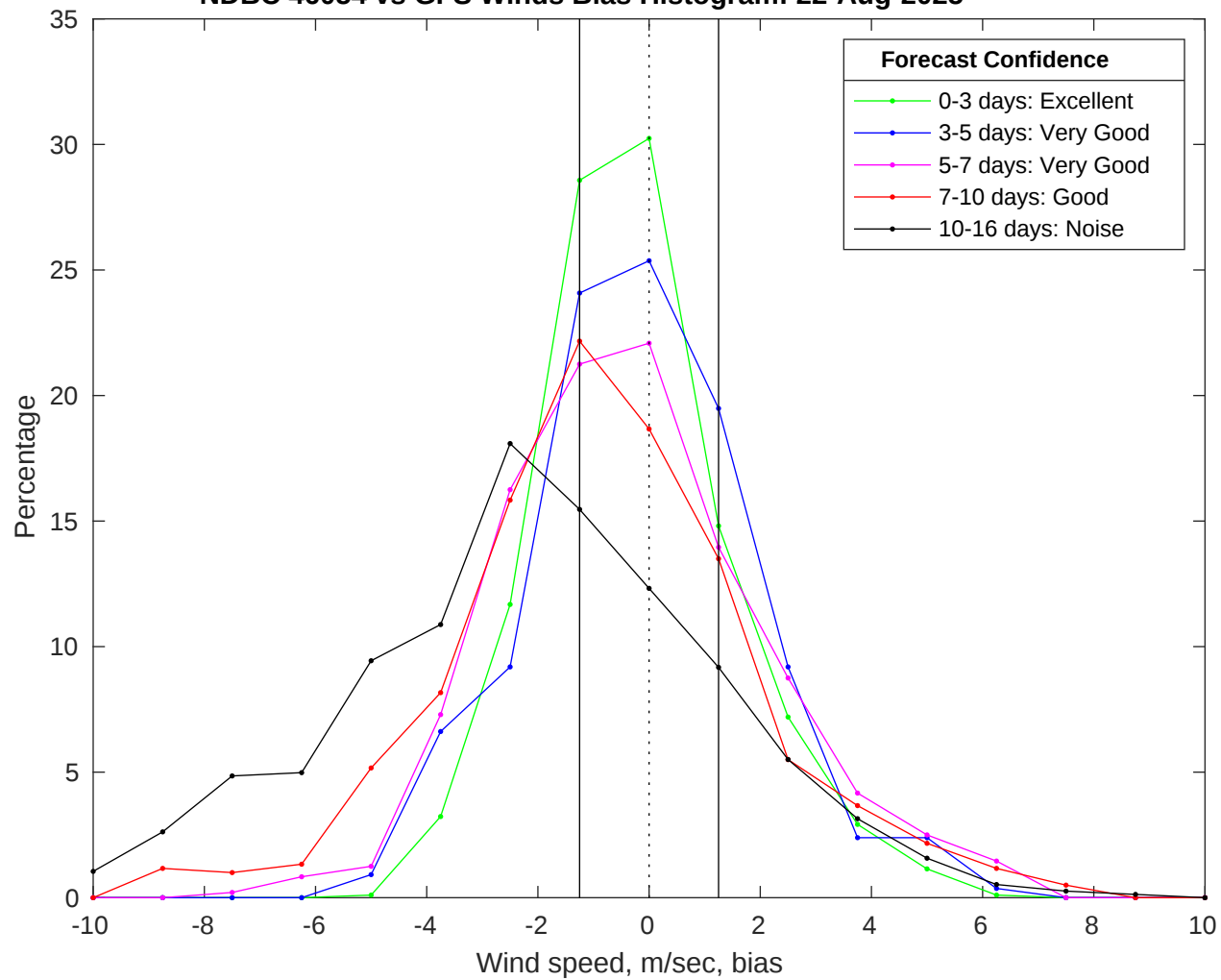
NDBC 46054 vs GFS Winds Bias Histogram: 22-Aug-2025
