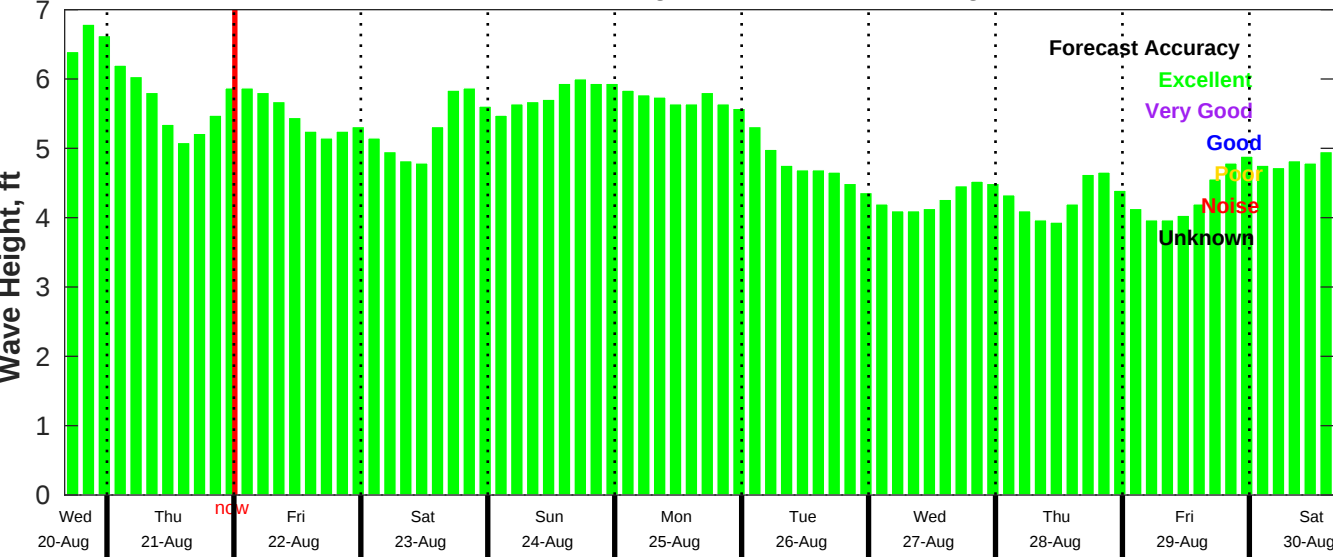
CMEMS Wave Forecast for NDBC 46054 from 20-Aug-2025 16:00:00 to 30-Aug-2025 16:00:00
