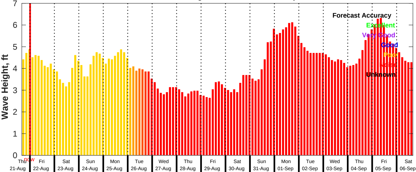
GFS Wave Forecast for NDBC 46054 from 21-Aug-2025 16:00:00 to 06-Sep-2025 16:00:00
