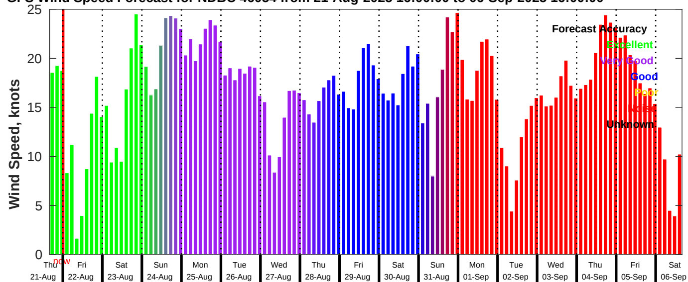
GFS Wind Speed Forecast for NDBC 46054 from 21-Aug-2025 16:00:00 to 06-Sep-2025 16:00:00
