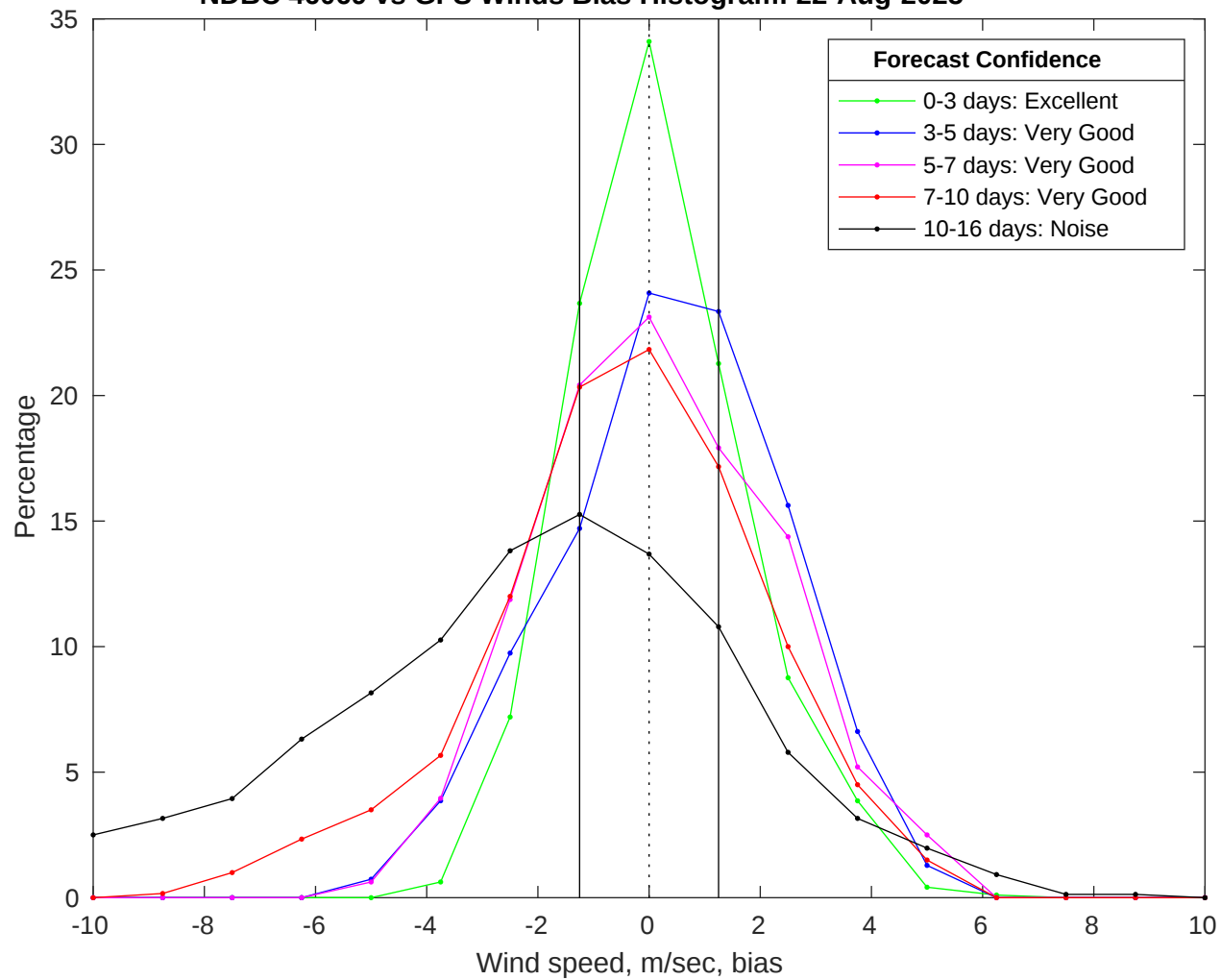
NDBC 46069 vs GFS Winds Bias Histogram: 22-Aug-2025
