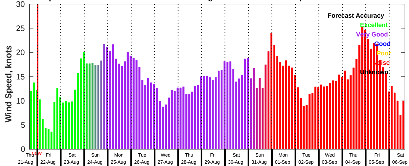
GFS Wind Speed Forecast for NDBC 46069 from 21-Aug-2025 16:00:00 to 06-Sep-2025 16:00:00
