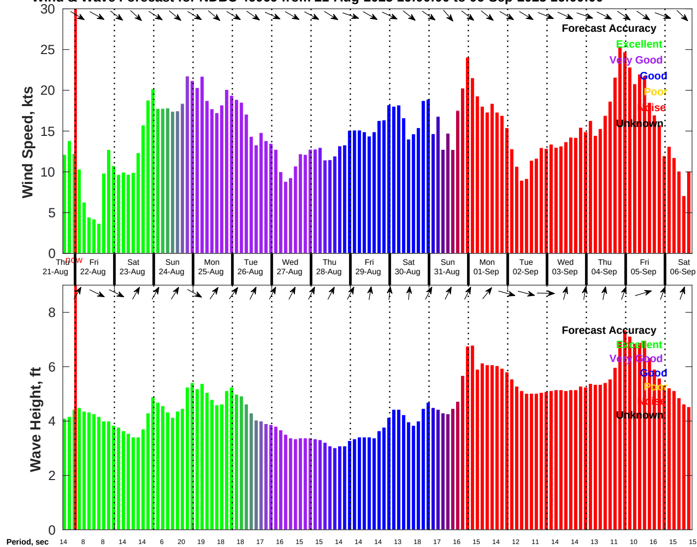
Wind & Wave Forecast for NDBC 46069 from 21-Aug-2025 16:00:00 to 06-Sep-2025 16:00:00
