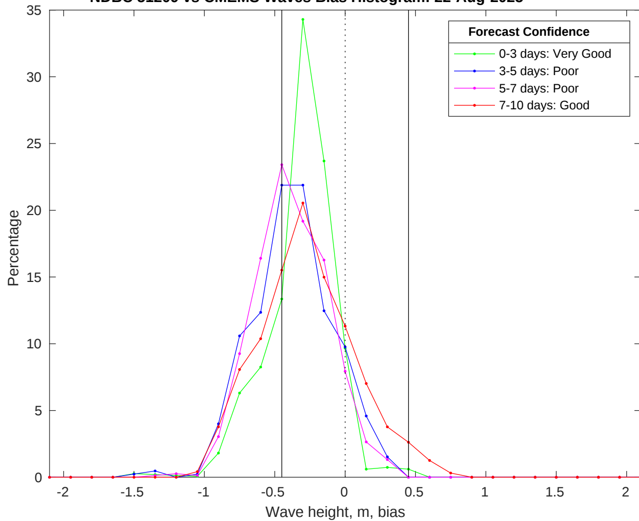
NDBC 51209 vs CMEMS Waves Bias Histogram: 22-Aug-2025
