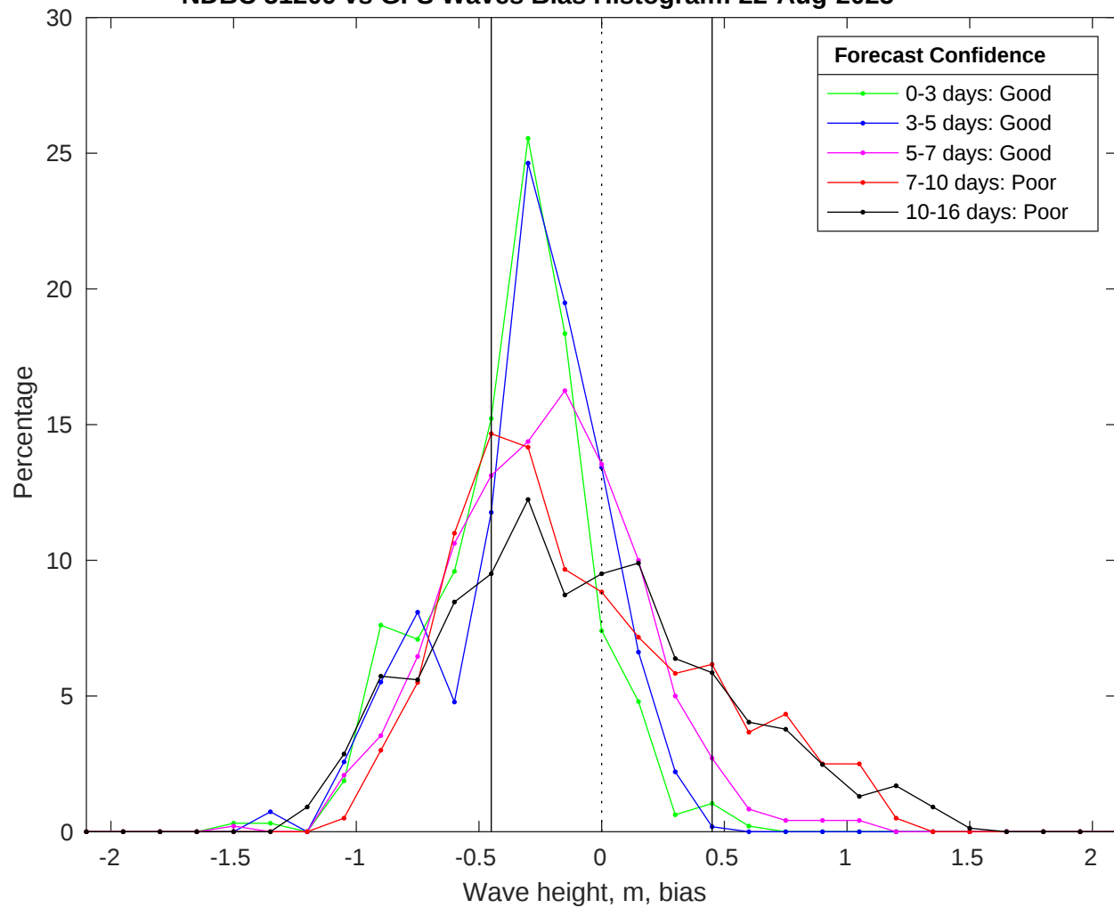
NDBC 51209 vs GFS Waves Bias Histogram: 22-Aug-2025
