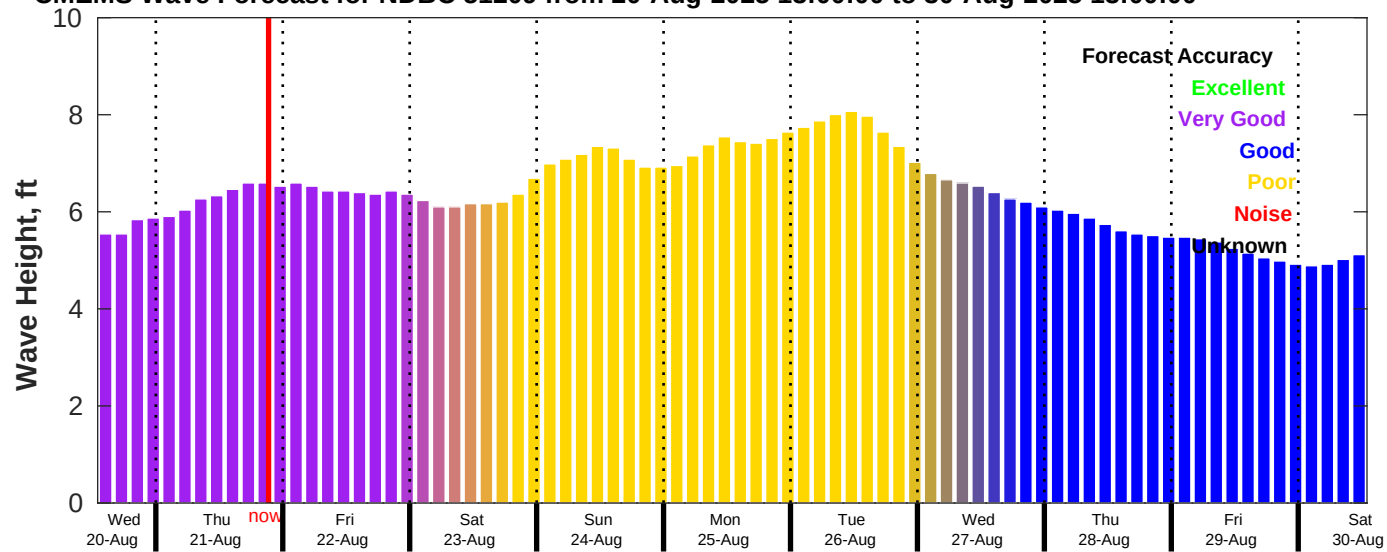
CMEMS Wave Forecast for NDBC 51209 from 20-Aug-2025 13:00:00 to 30-Aug-2025 13:00:00
