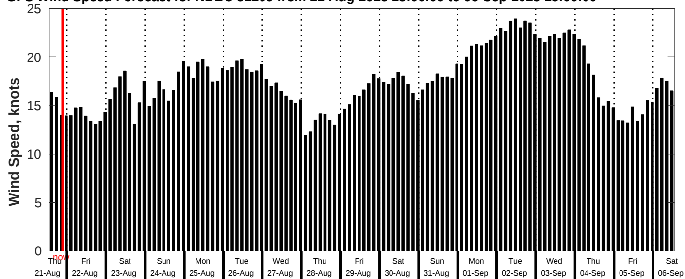
GFS Wind Speed Forecast for NDBC 51209 from 21-Aug-2025 13:00:00 to 06-Sep-2025 13:00:00
