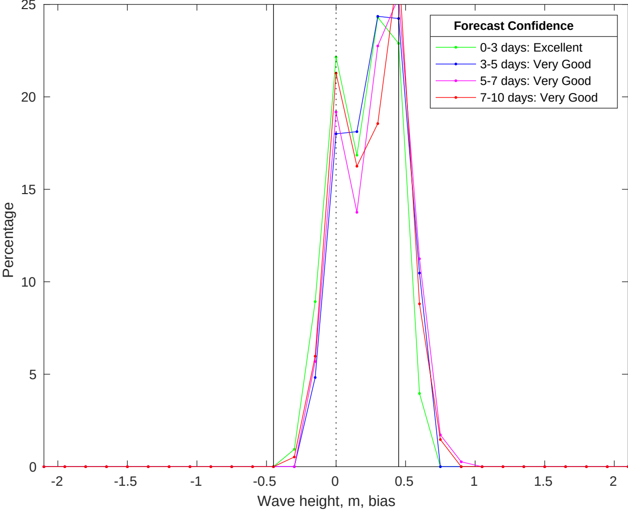
NDBC 51211 vs CMEMS Waves Bias Histogram: 22-Aug-2025
