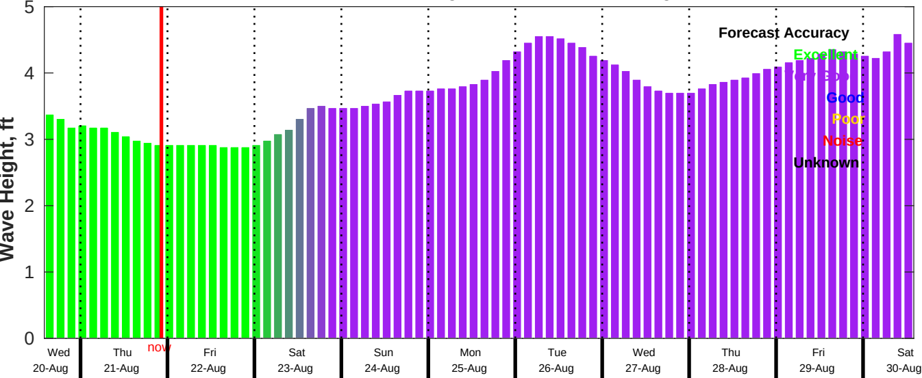
CMEMS Wave Forecast for NDBC 51211 from 20-Aug-2025 14:00:00 to 30-Aug-2025 14:00:00
