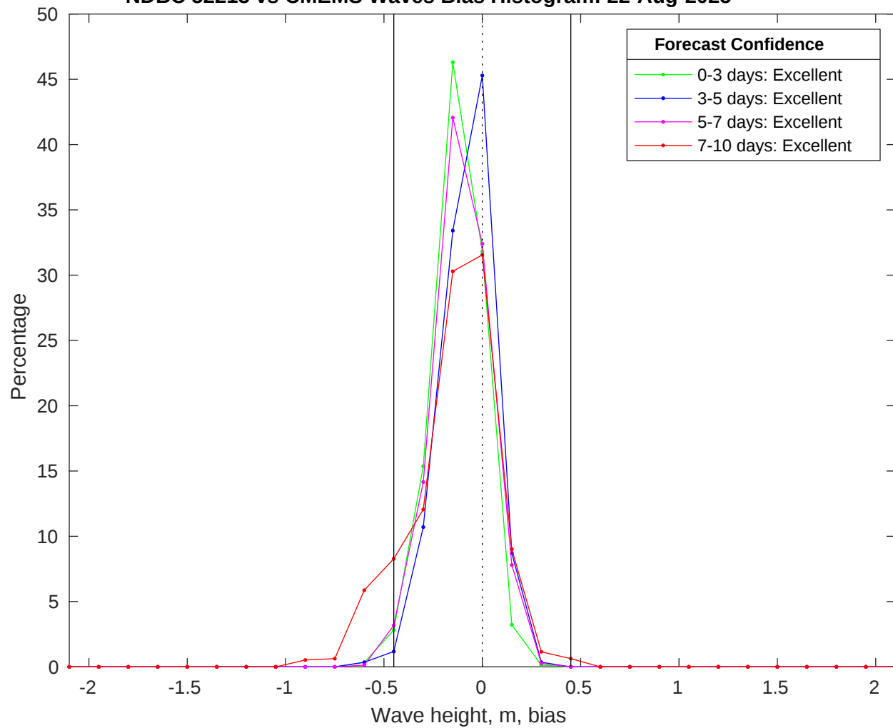
NDBC 52213 vs CMEMS Waves Bias Histogram: 22-Aug-2025
