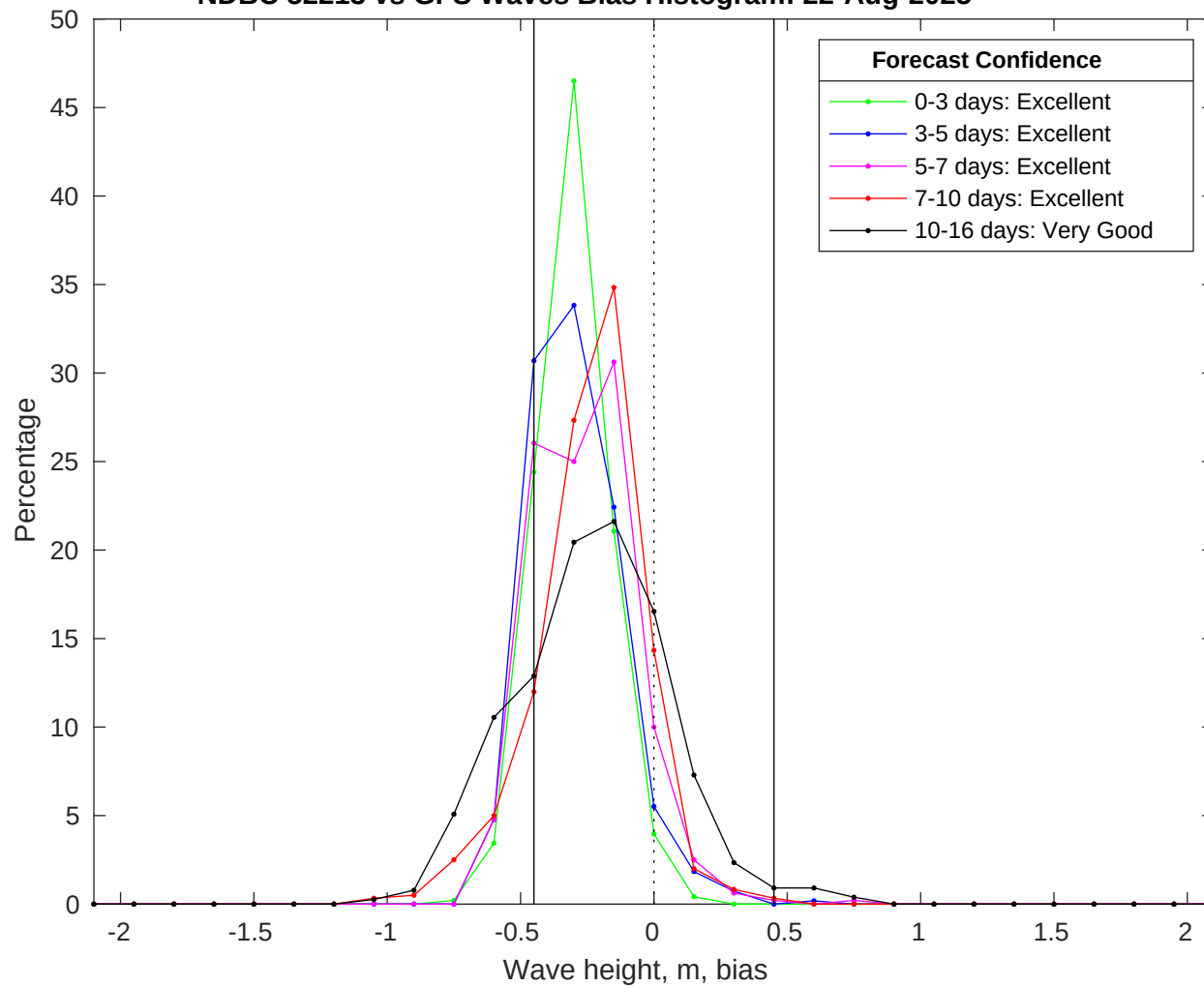
NDBC 52213 vs GFS Waves Bias Histogram: 22-Aug-2025
