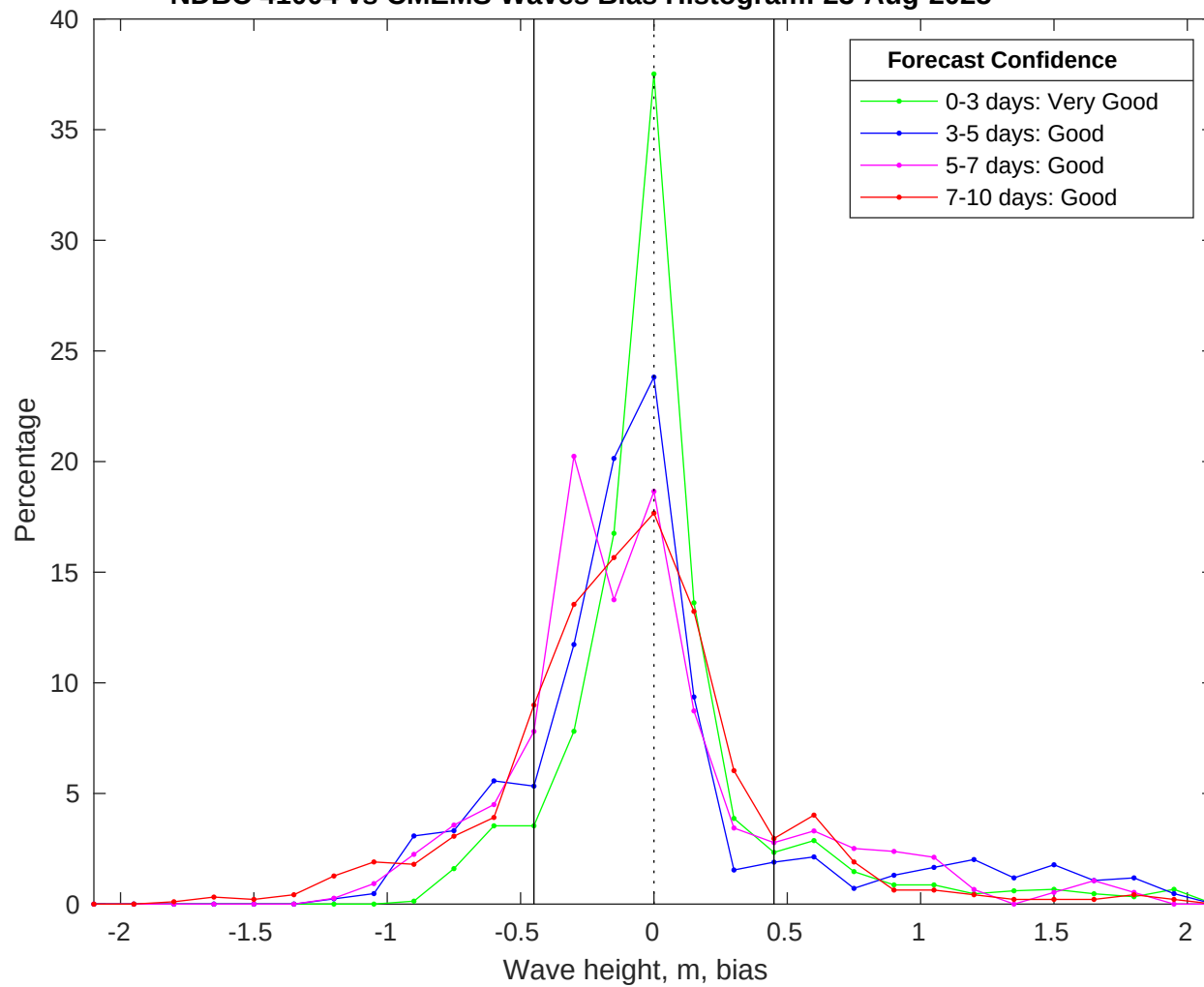
NDBC 41004 vs CMEMS Waves Bias Histogram: 23-Aug-2025
