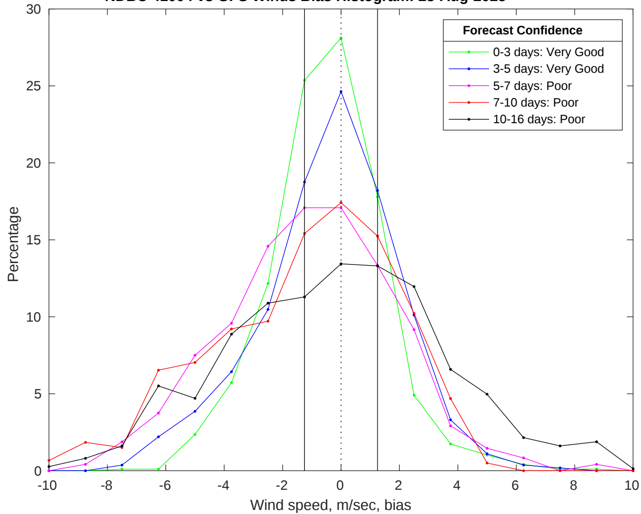
NDBC 41004 vs GFS Winds Bias Histogram: 23-Aug-2025
