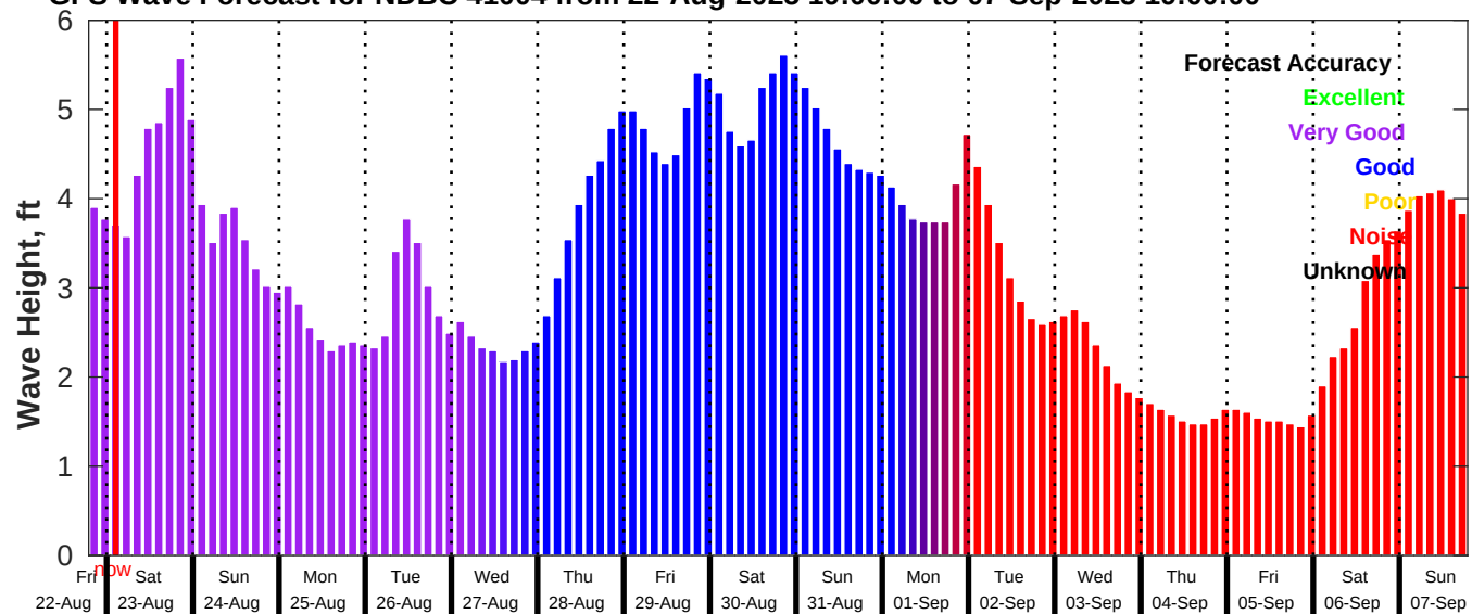
GFS Wave Forecast for NDBC 41004 from 22-Aug-2025 19:00:00 to 07-Sep-2025 19:00:00
