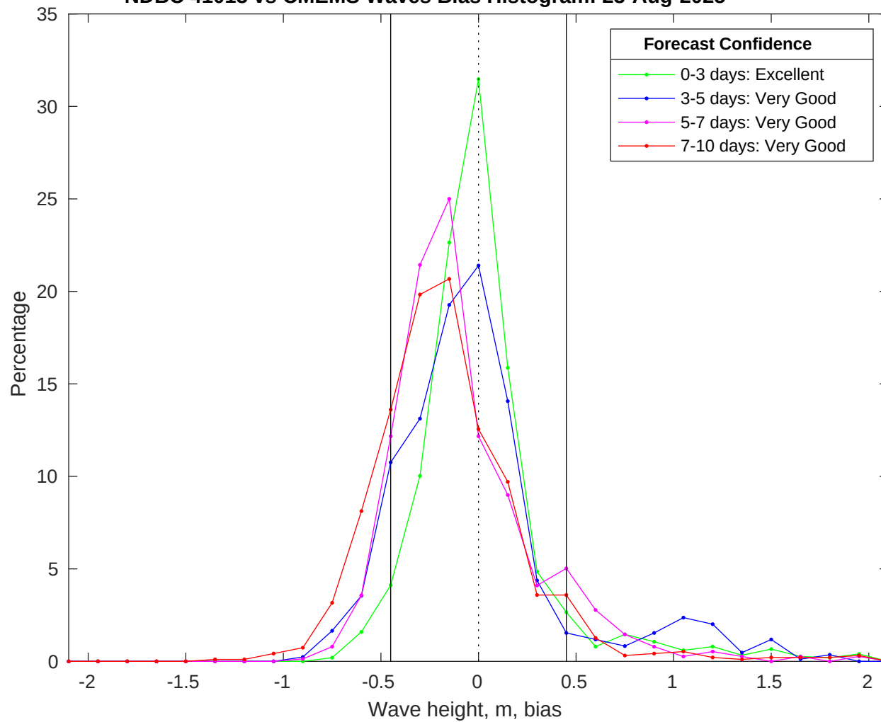
NDBC 41013 vs CMEMS Waves Bias Histogram: 23-Aug-2025
