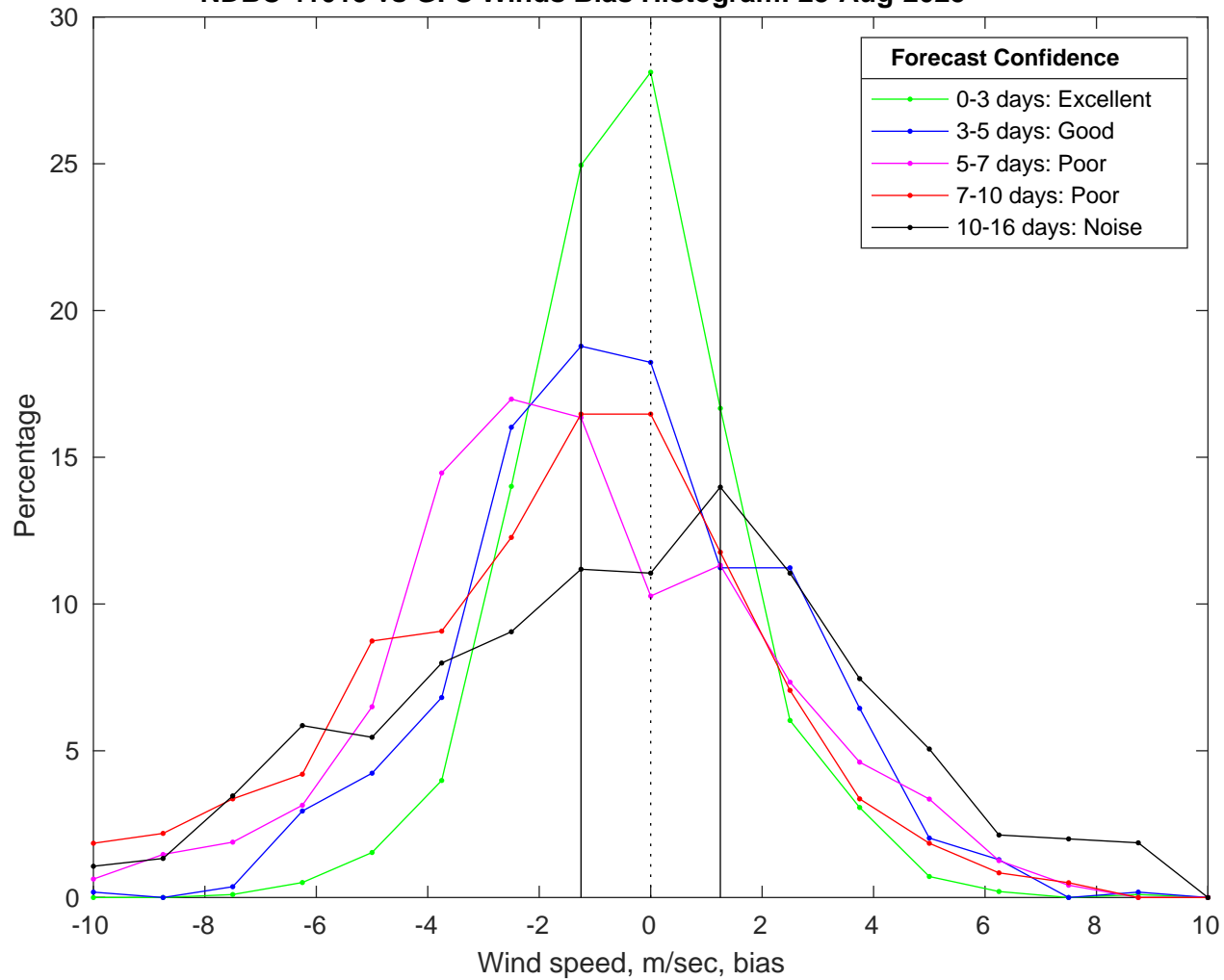
NDBC 41013 vs GFS Winds Bias Histogram: 23-Aug-2025
