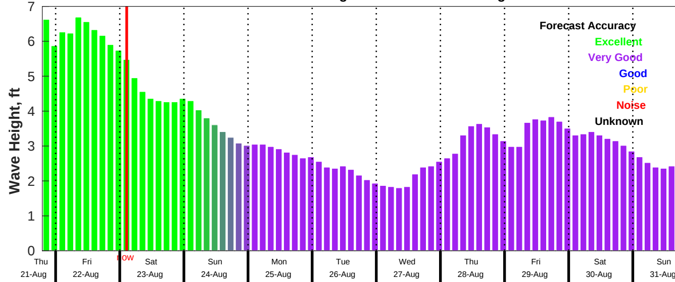
CMEMS Wave Forecast for NDBC 41013 from 21-Aug-2025 19:00:00 to 31-Aug-2025 19:00:00
