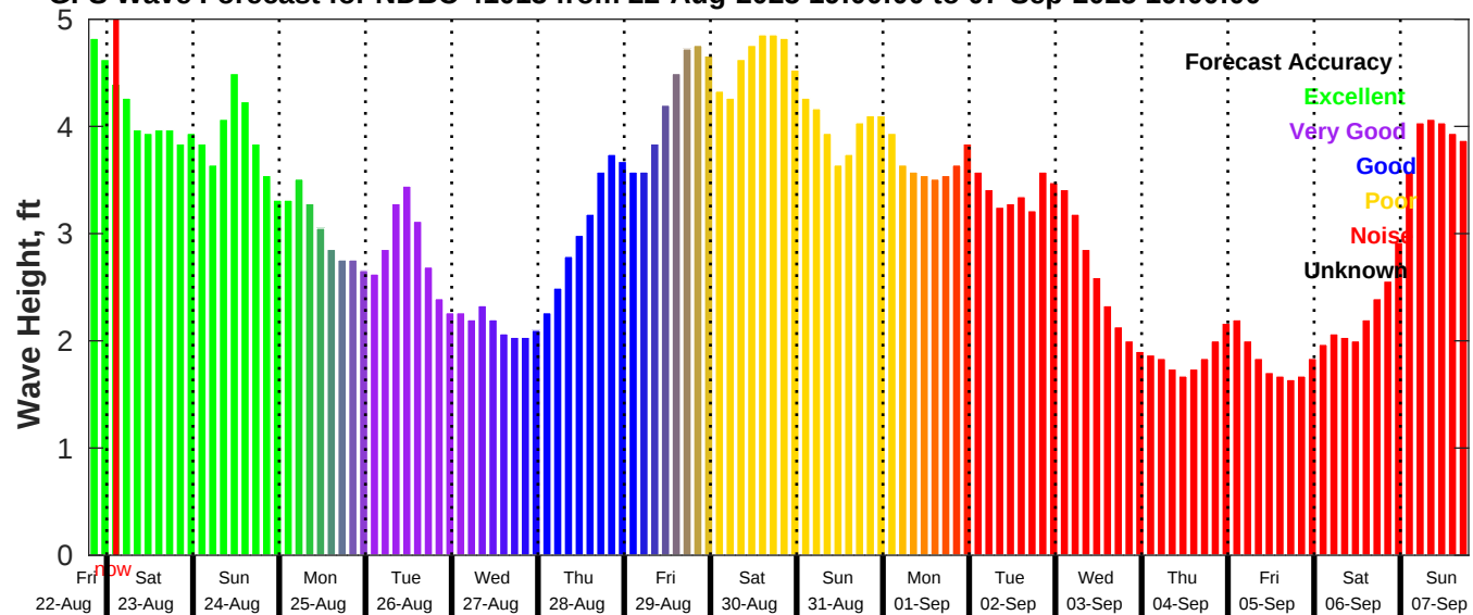
GFS Wave Forecast for NDBC 41013 from 22-Aug-2025 19:00:00 to 07-Sep-2025 19:00:00
