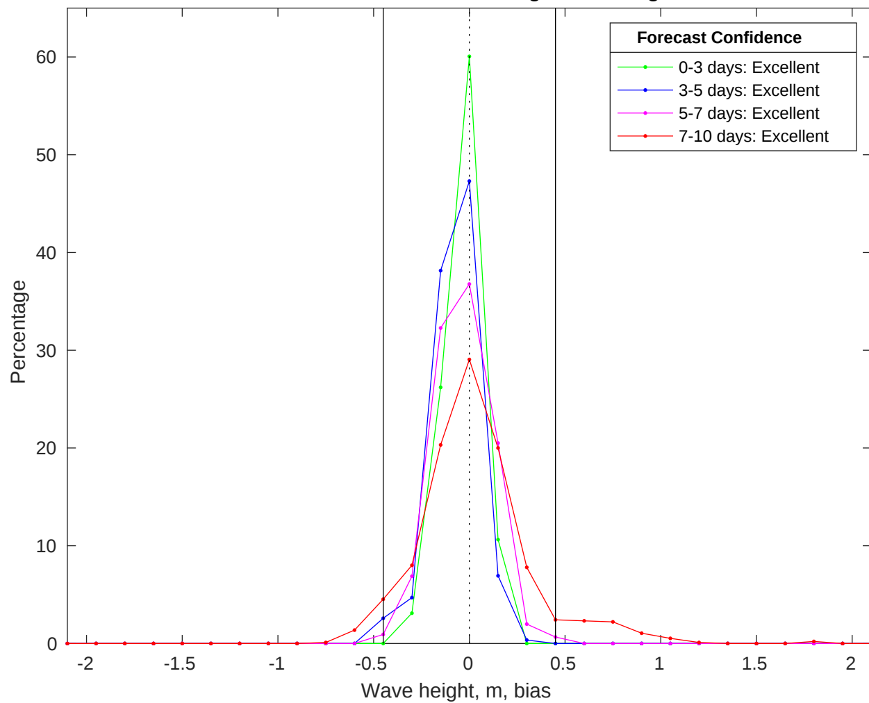
NDBC 41040 vs CMEMS Waves Bias Histogram: 23-Aug-2025
