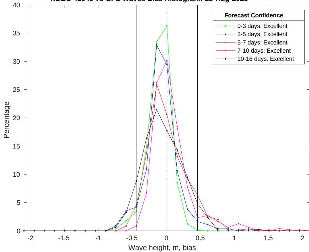
NDBC 41040 vs GFS Waves Bias Histogram: 23-Aug-2025
