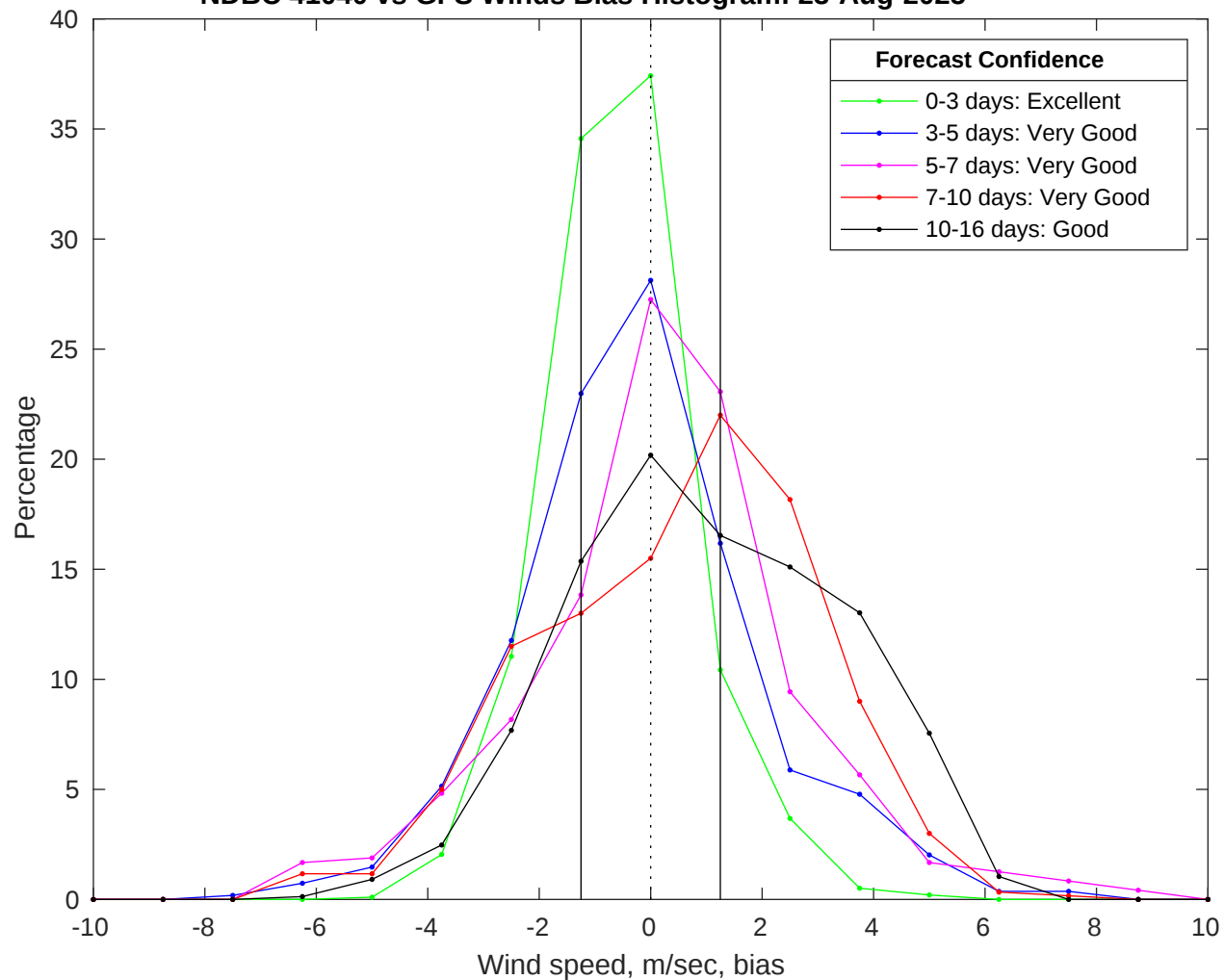
NDBC 41040 vs GFS Winds Bias Histogram: 23-Aug-2025
