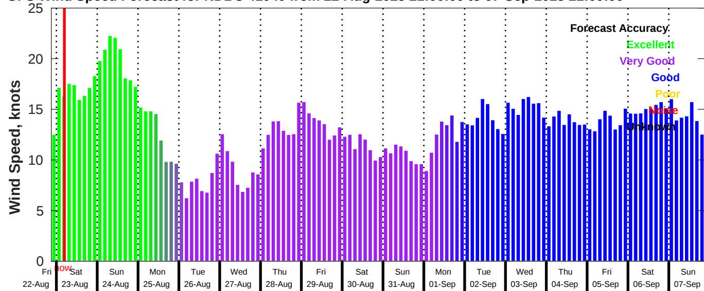
GFS Wind Speed Forecast for NDBC 41040 from 22-Aug-2025 21:00:00 to 07-Sep-2025 21:00:00
