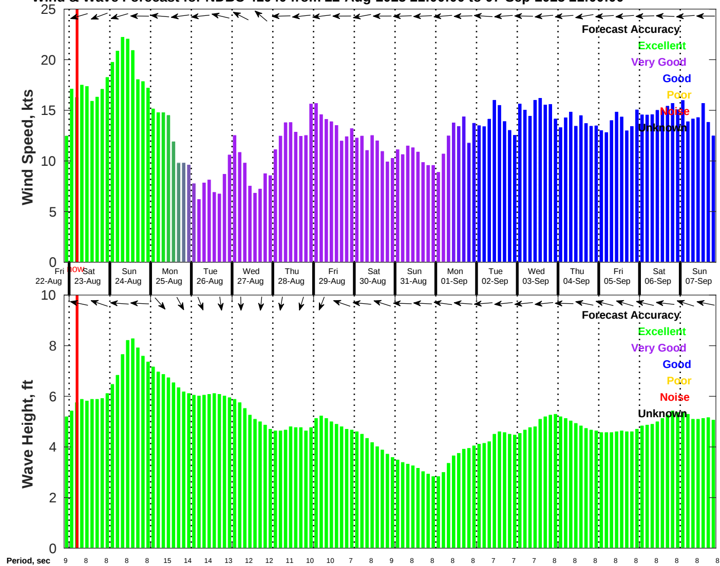
Wind & Wave Forecast for NDBC 41040 from 22-Aug-2025 21:00:00 to 07-Sep-2025 21:00:00
