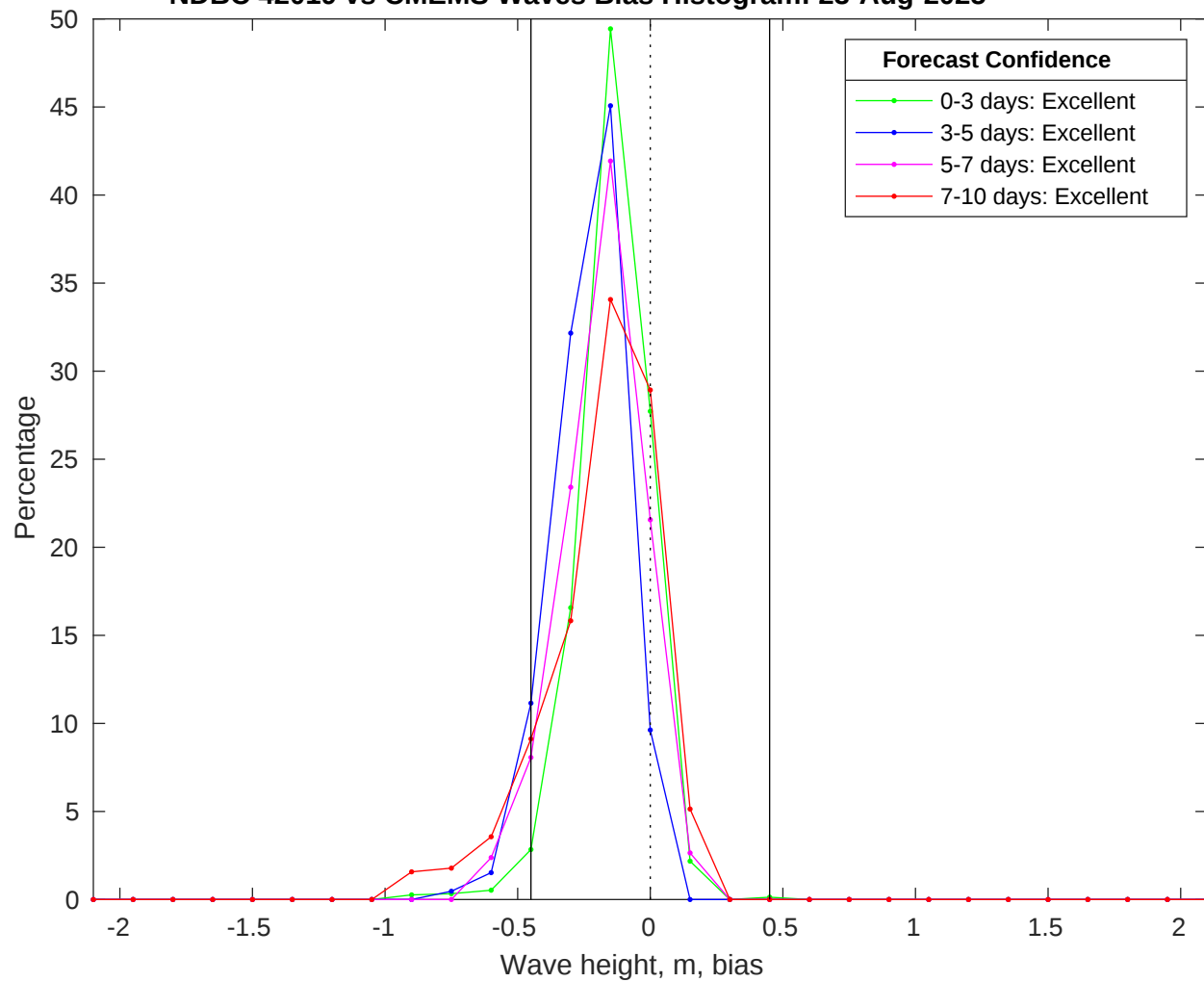
NDBC 42019 vs CMEMS Waves Bias Histogram: 23-Aug-2025
