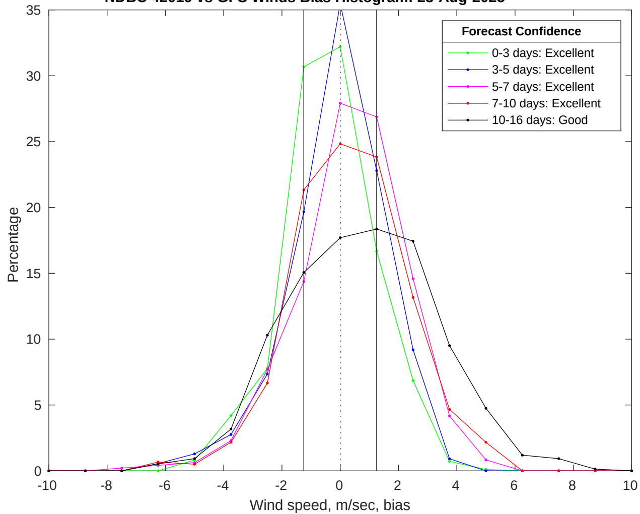
NDBC 42019 vs GFS Winds Bias Histogram: 23-Aug-2025
