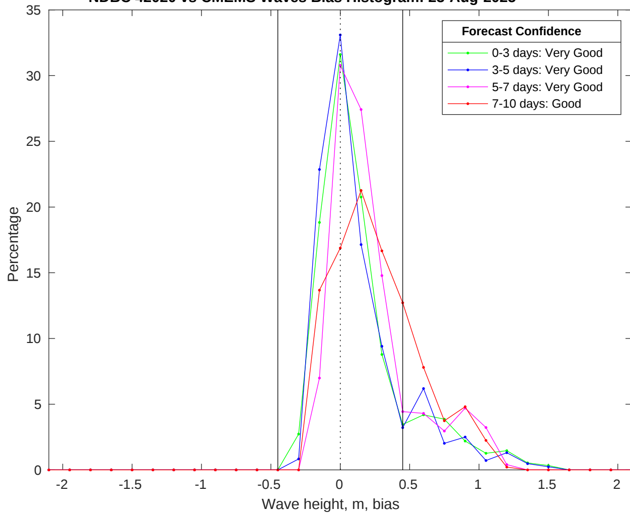
NDBC 42020 vs CMEMS Waves Bias Histogram: 23-Aug-2025
