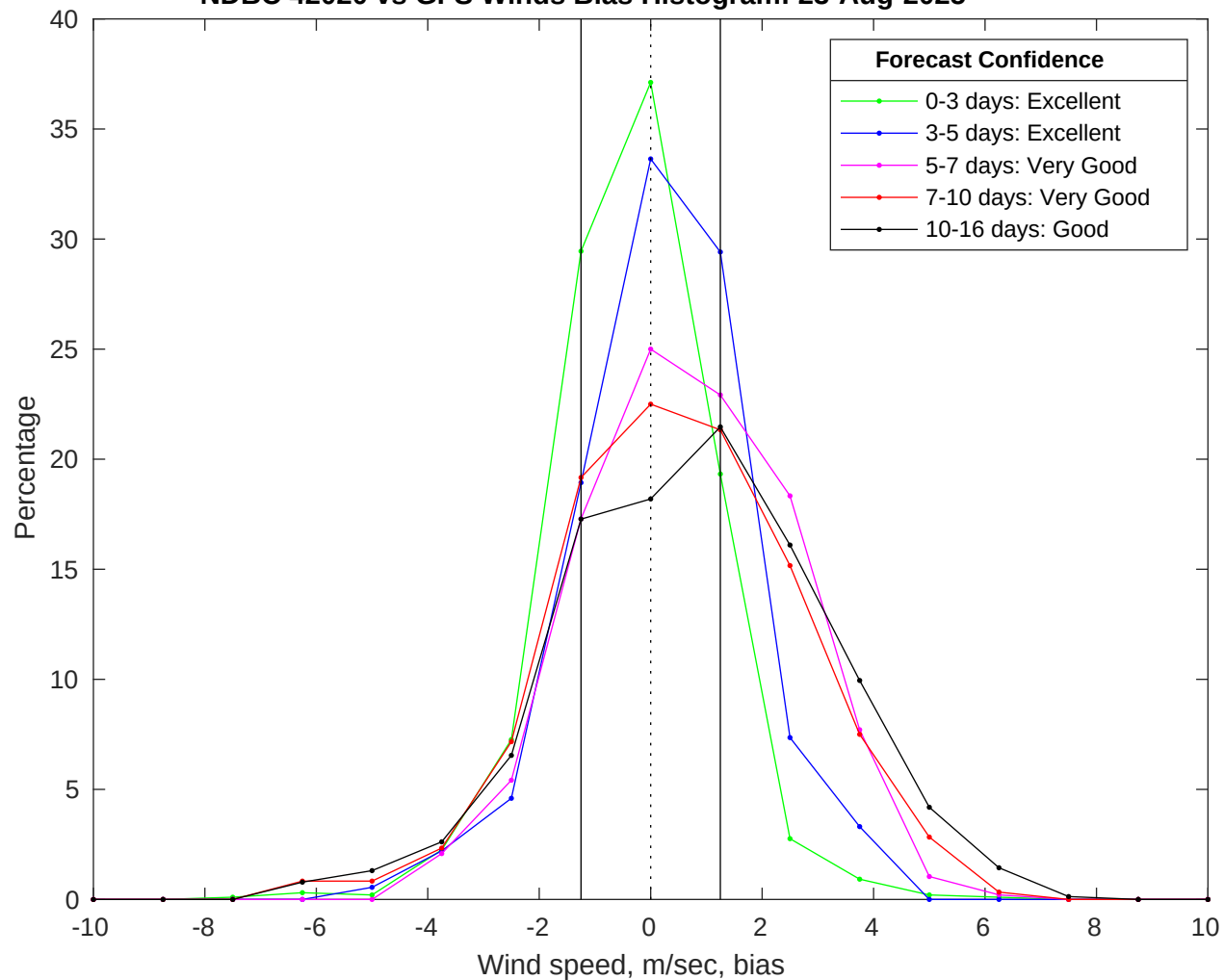
NDBC 42020 vs GFS Winds Bias Histogram: 23-Aug-2025
