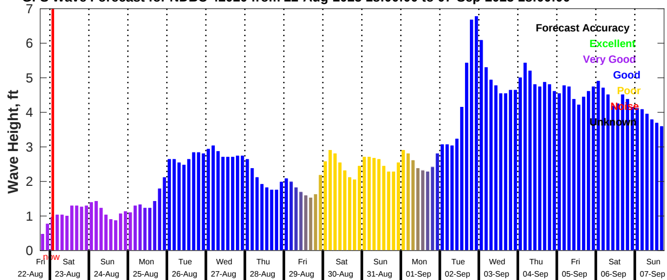
GFS Wave Forecast for NDBC 42020 from 22-Aug-2025 18:00:00 to 07-Sep-2025 18:00:00
