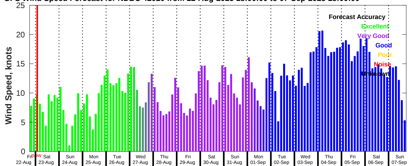
GFS Wind Speed Forecast for NDBC 42020 from 22-Aug-2025 18:00:00 to 07-Sep-2025 18:00:00
