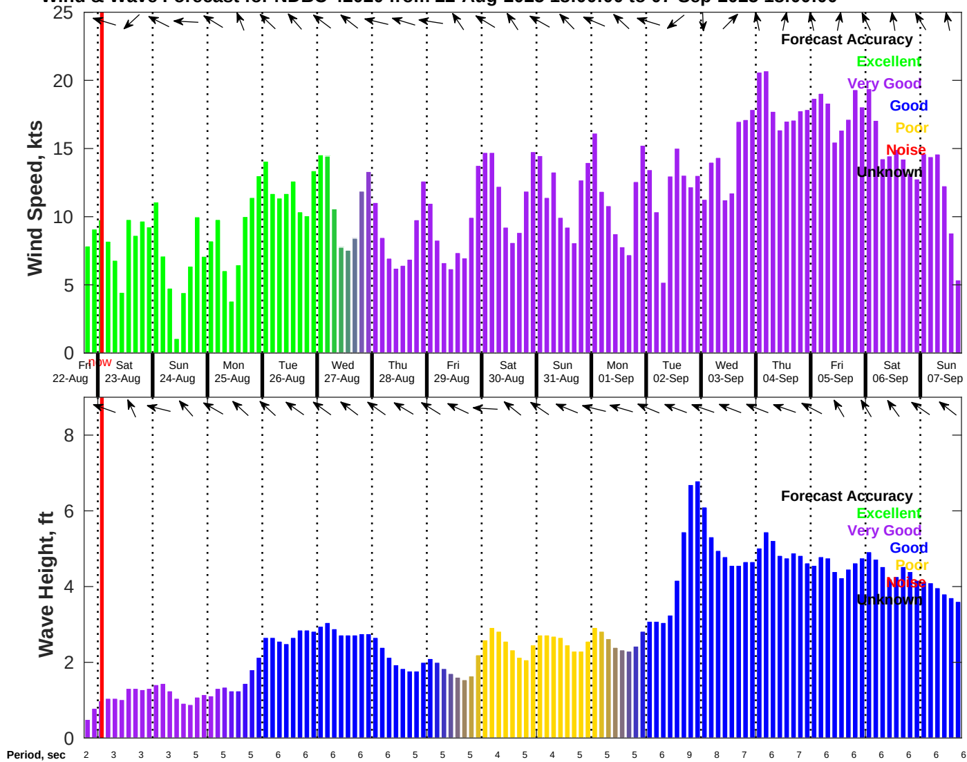
Wind & Wave Forecast for NDBC 42020 from 22-Aug-2025 18:00:00 to 07-Sep-2025 18:00:00
