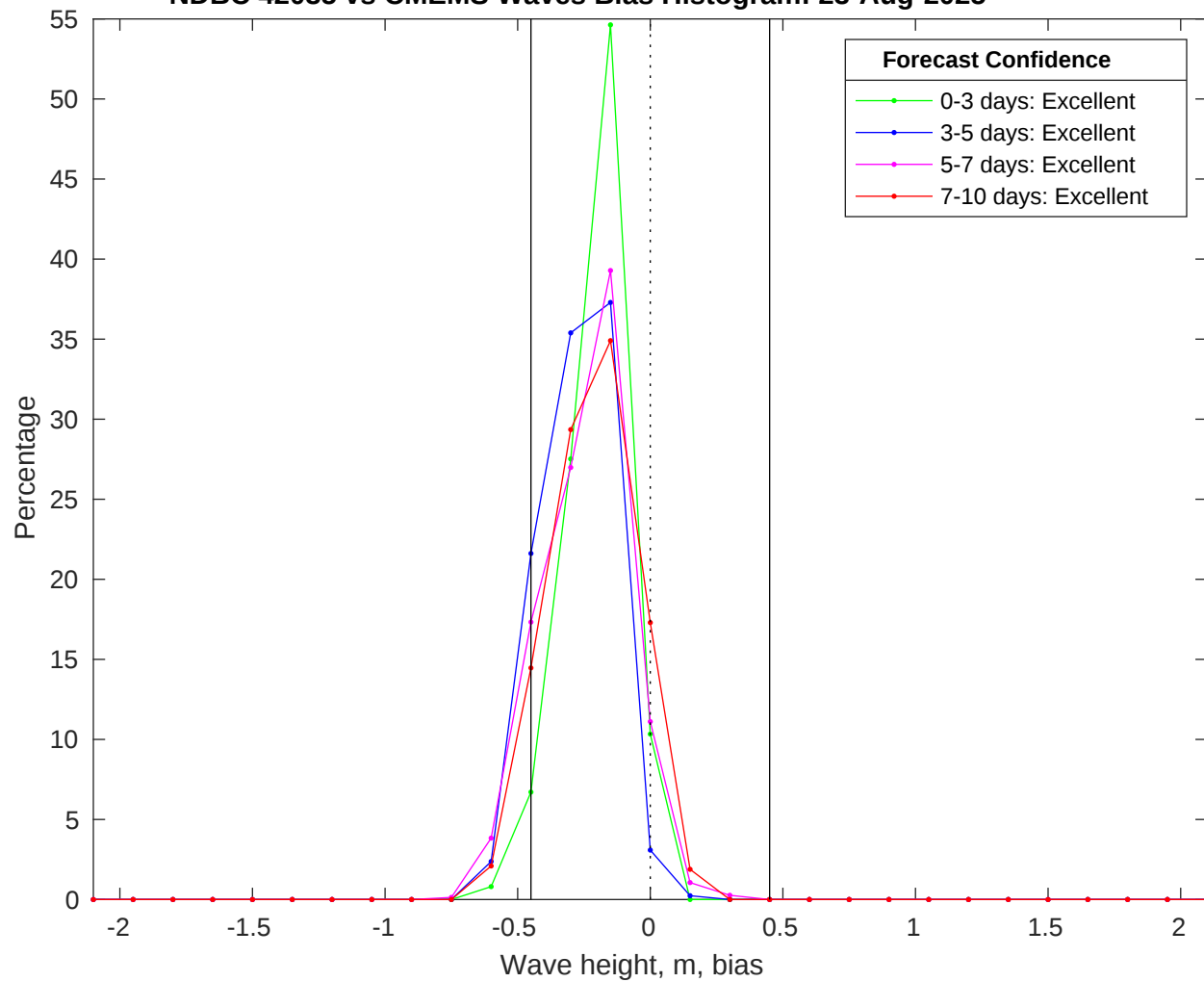
NDBC 42035 vs CMEMS Waves Bias Histogram: 23-Aug-2025
