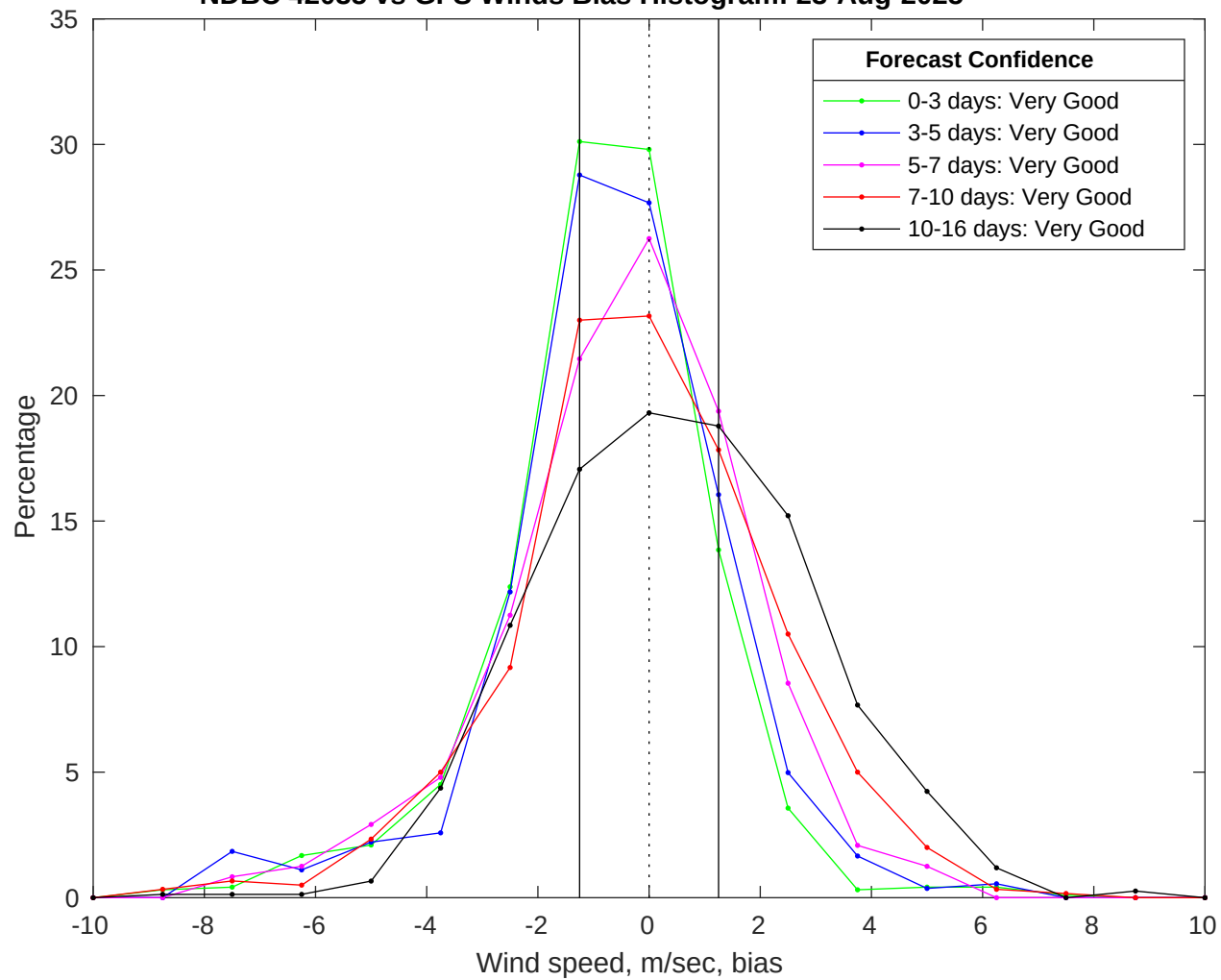
NDBC 42035 vs GFS Winds Bias Histogram: 23-Aug-2025
