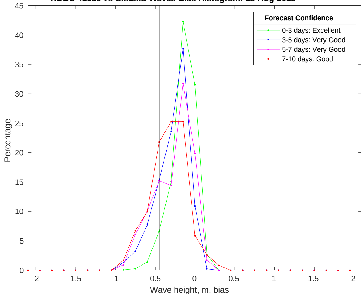
NDBC 42036 vs CMEMS Waves Bias Histogram: 23-Aug-2025
