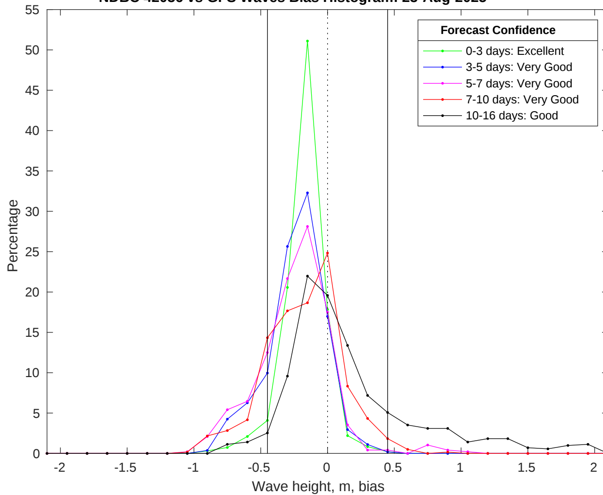
NDBC 42036 vs GFS Waves Bias Histogram: 23-Aug-2025
