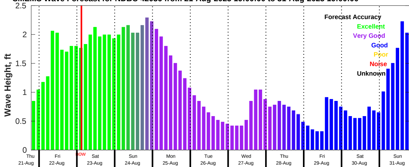
CMEMS Wave Forecast for NDBC 42036 from 21-Aug-2025 19:00:00 to 31-Aug-2025 19:00:00
