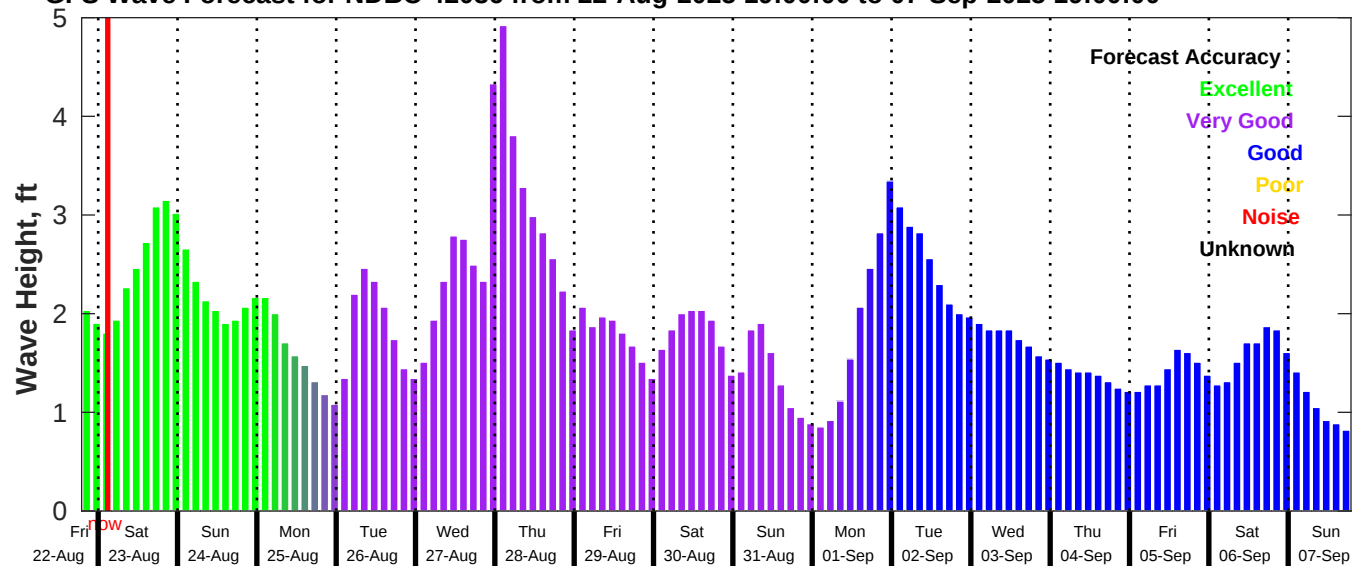
GFS Wave Forecast for NDBC 42036 from 22-Aug-2025 19:00:00 to 07-Sep-2025 19:00:00
