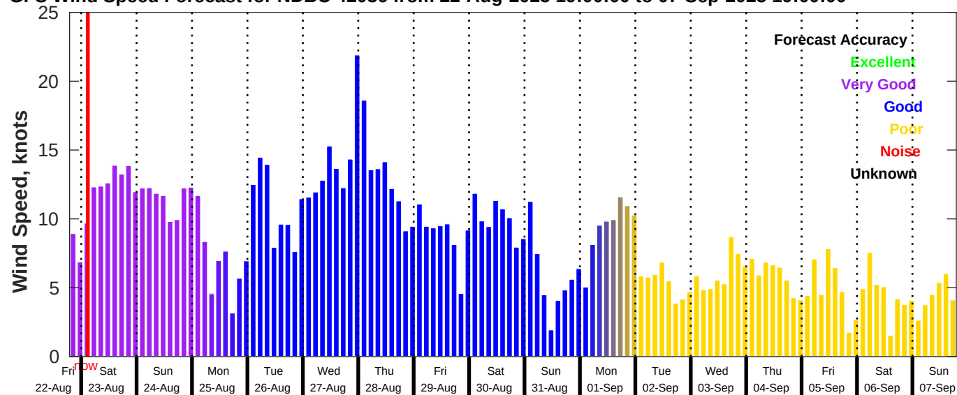
GFS Wind Speed Forecast for NDBC 42036 from 22-Aug-2025 19:00:00 to 07-Sep-2025 19:00:00
