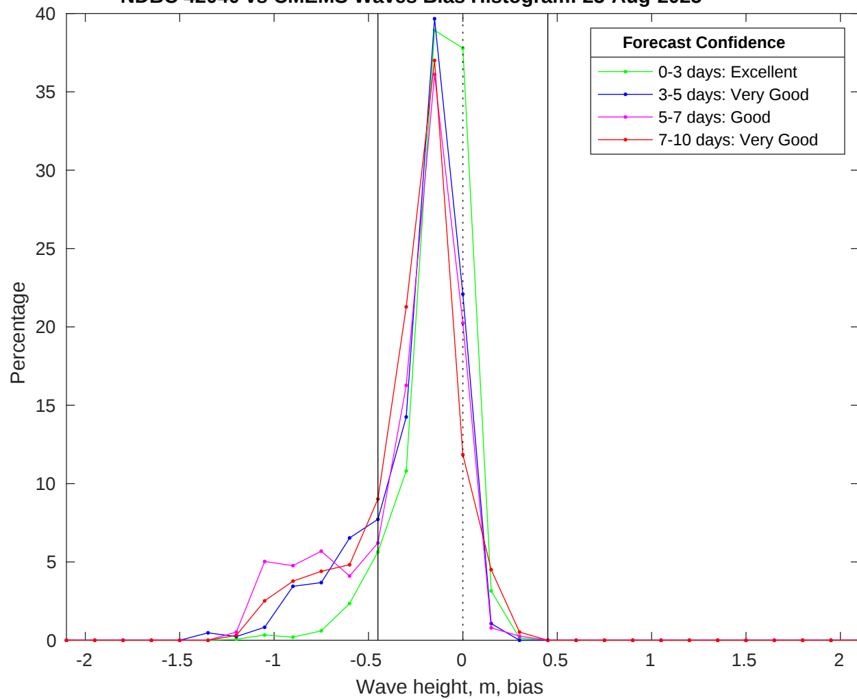
NDBC 42040 vs CMEMS Waves Bias Histogram: 23-Aug-2025
