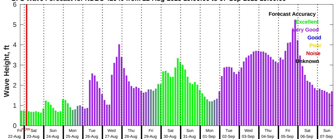
GFS Wave Forecast for NDBC 42040 from 22-Aug-2025 19:00:00 to 07-Sep-2025 19:00:00
