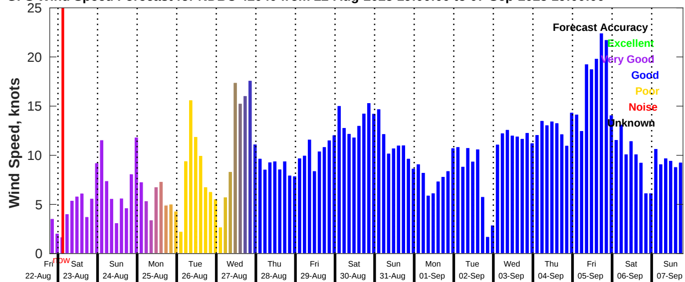
GFS Wind Speed Forecast for NDBC 42040 from 22-Aug-2025 19:00:00 to 07-Sep-2025 19:00:00
