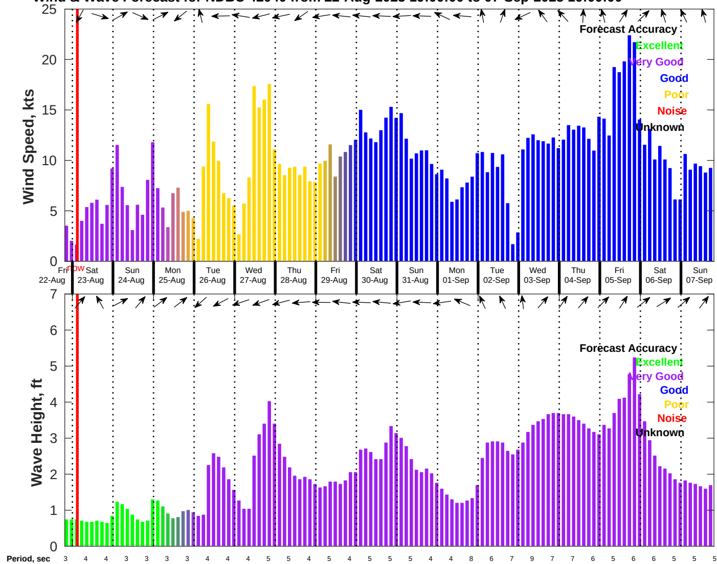
Wind & Wave Forecast for NDBC 42040 from 22-Aug-2025 19:00:00 to 07-Sep-2025 19:00:00
